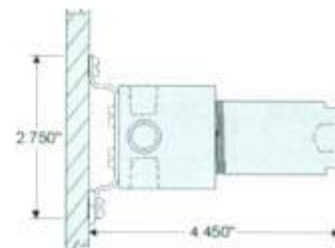
Horizontal Mounting
