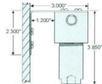
Vertical Mounting
